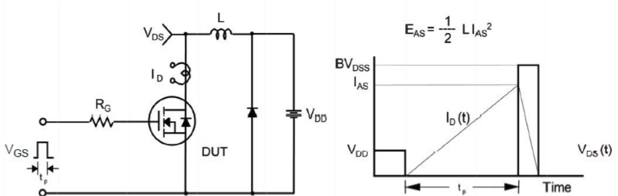
Unclamped Inductive Switching Test Circuit &amp; Waveforms
