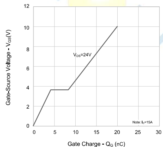
Figure 6. Gate Charge
